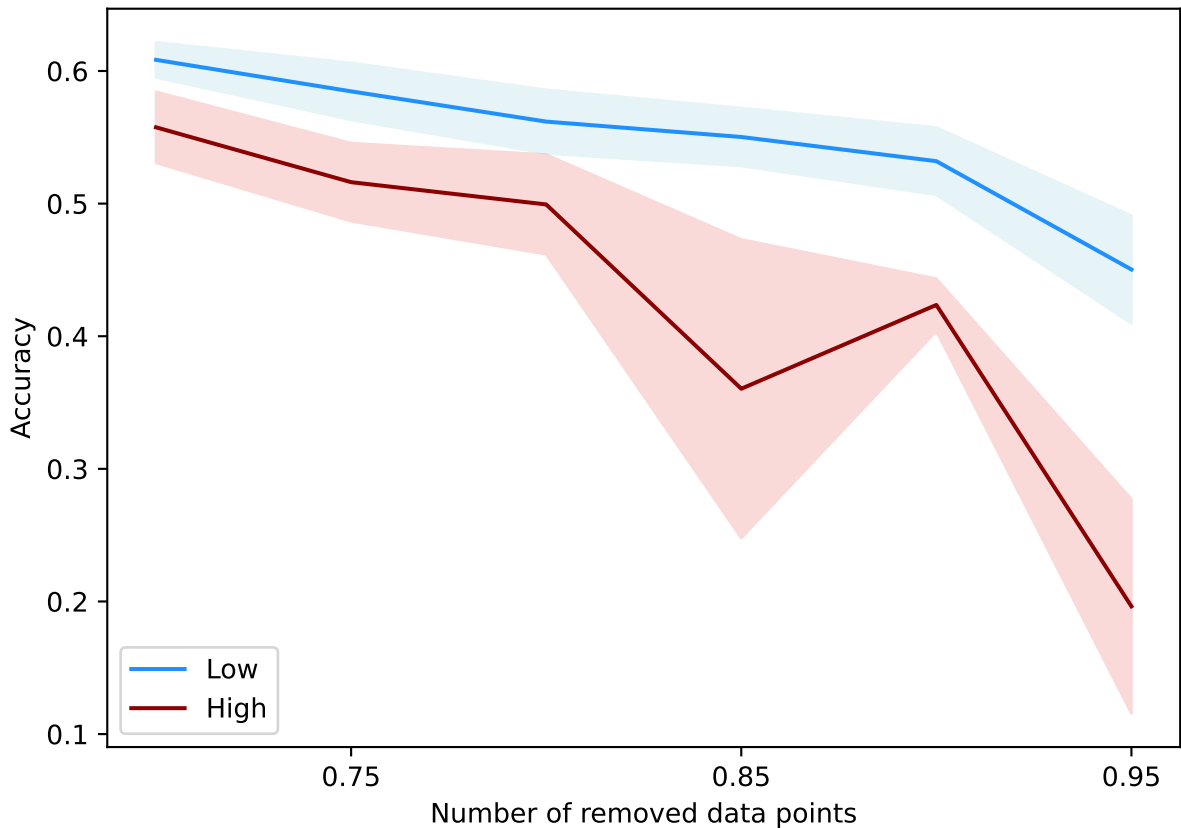
DataAttrOpt(5000, 0.02, 15, max+s, alpha=0.5) - cifar10-embeddings
